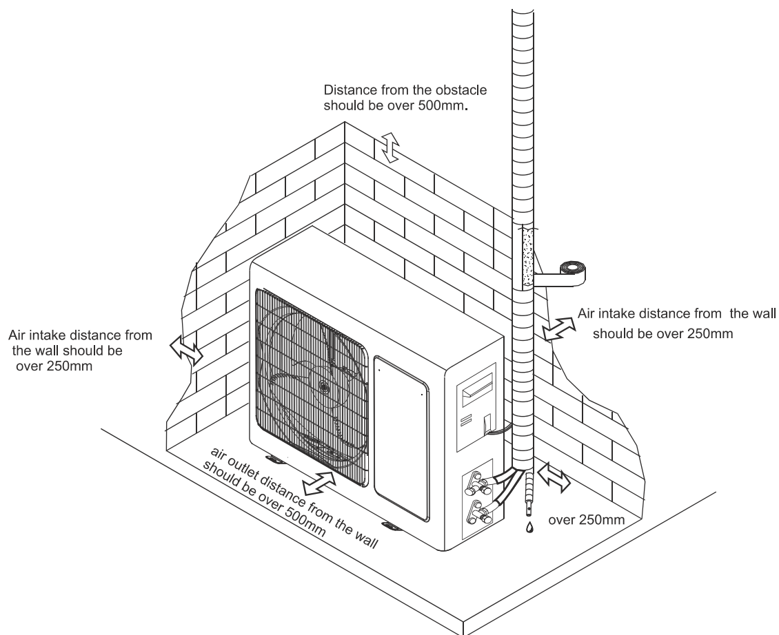
outdoor unit
