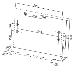
Schematic drawing of hooks:
