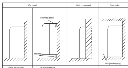
Location for securing the installation panel.
